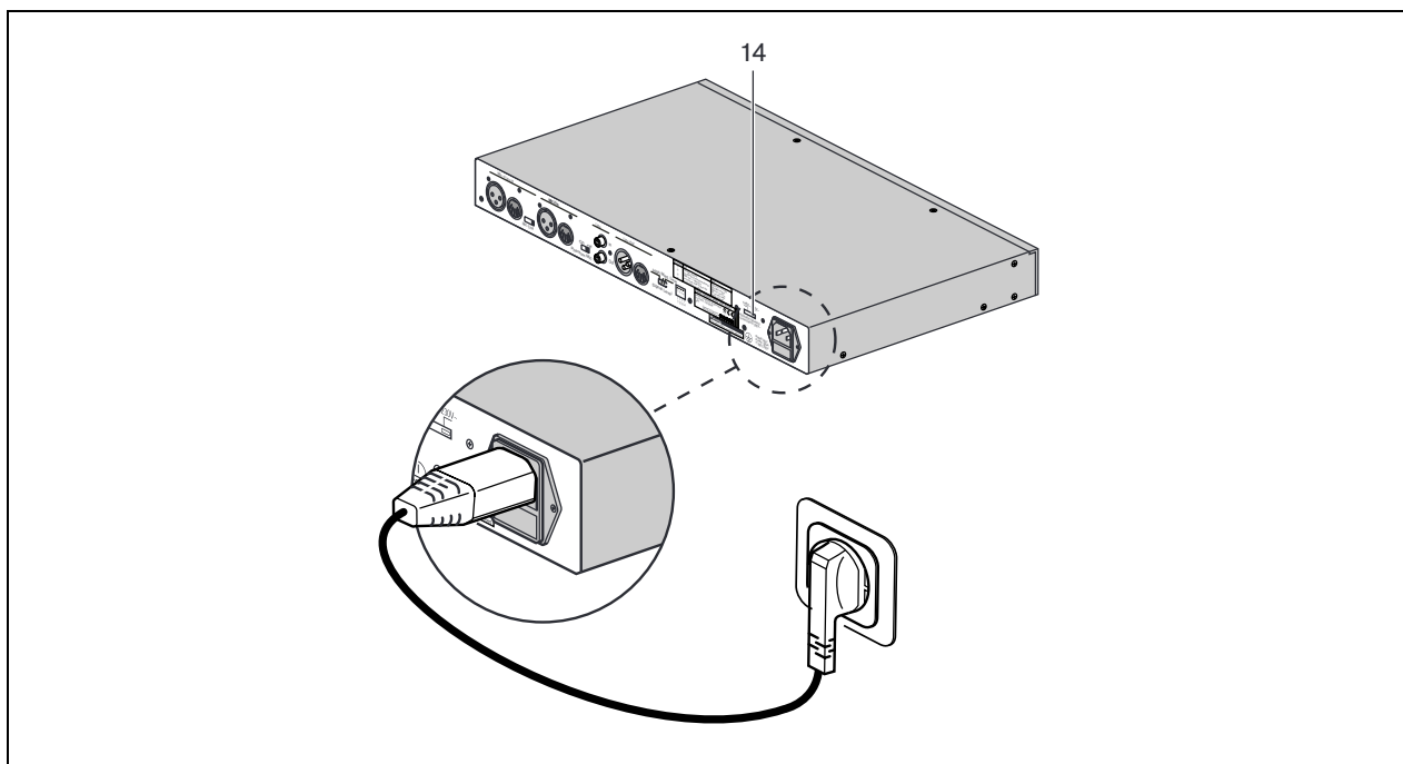
figure 3.7: Mains connection
