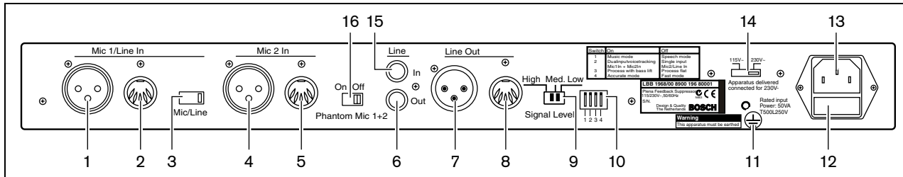
figure 1.3: Controls and connections (rear)
