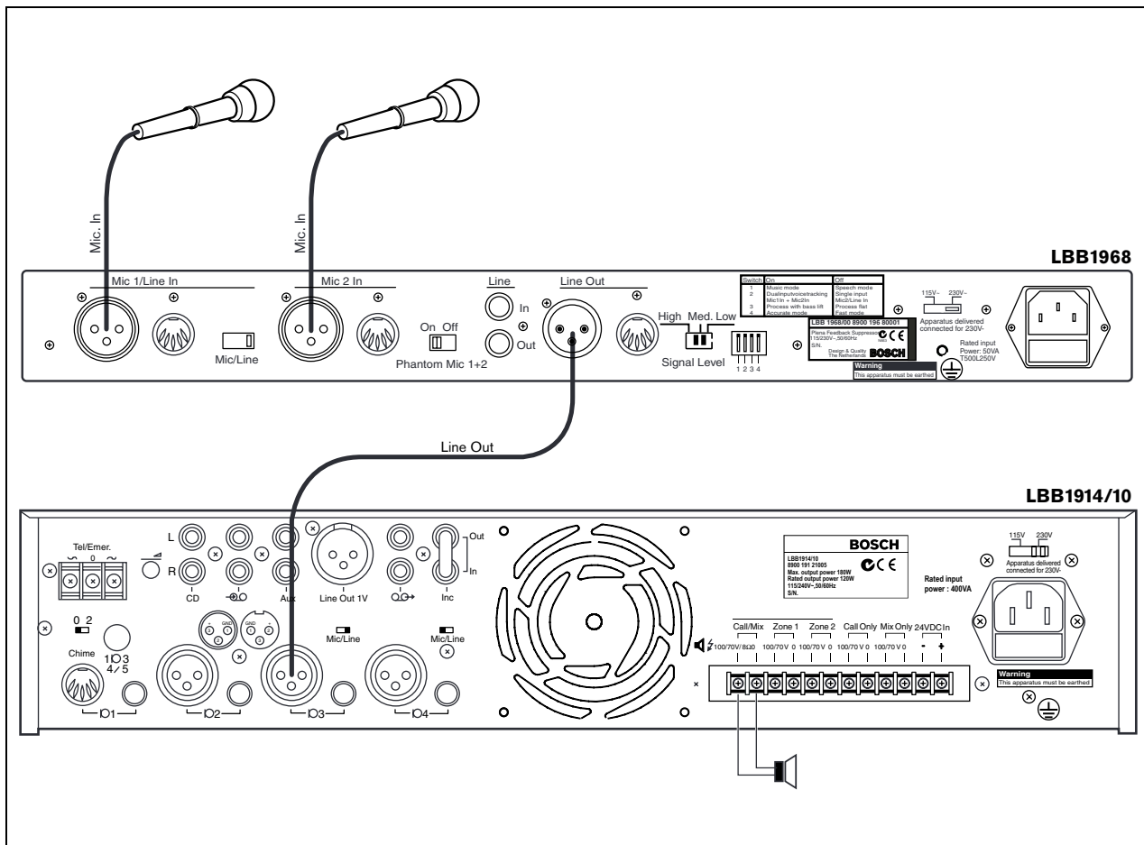
figure 3.4: Presentation set-up
