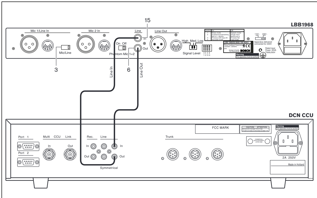
figure 3.3: Conference set-up
