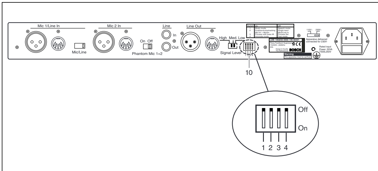
figure 3.6: Options switches
