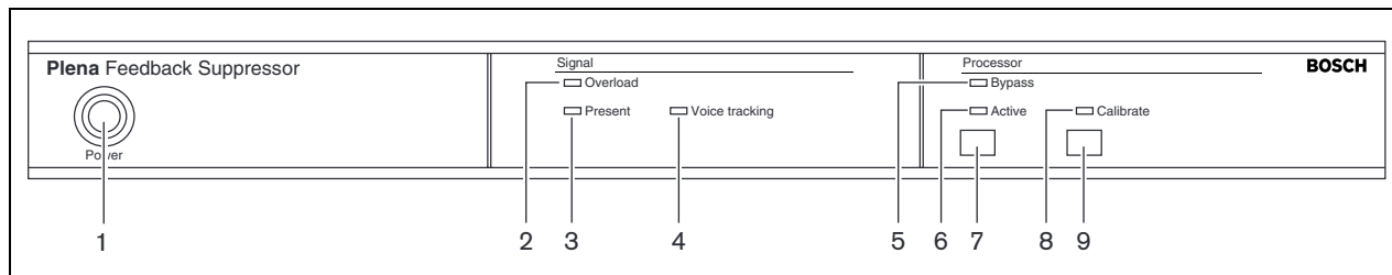
figure 4.1: Controls and indicators (front)
