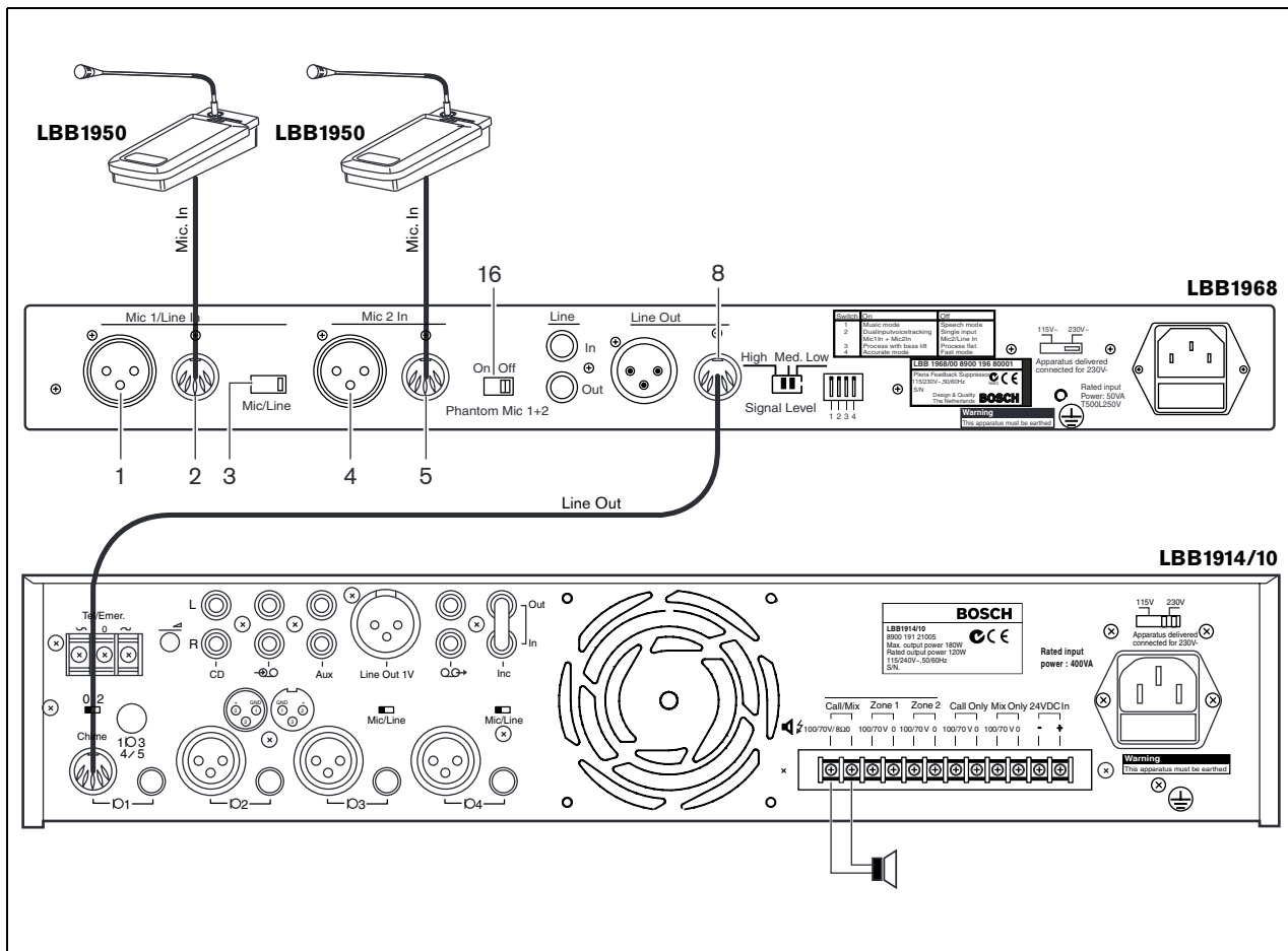
figure 3.1: Announcement set-up
