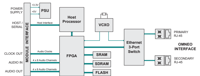
Fig. 1: Circuit diagram
